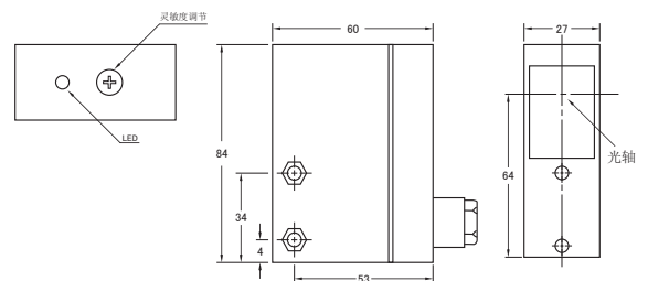
图194 HDT500-27K-□ HDM80-27K-□ HDR200-27K-□
