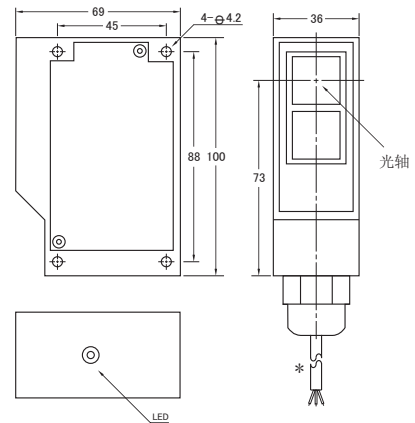
图194 HDT500-27K-□ HDM80-27K-□ HDR200-27K-□
