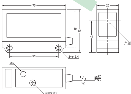
图193 HDT500-26K-□ HDM80-26K-□ HDR200-26K-□
