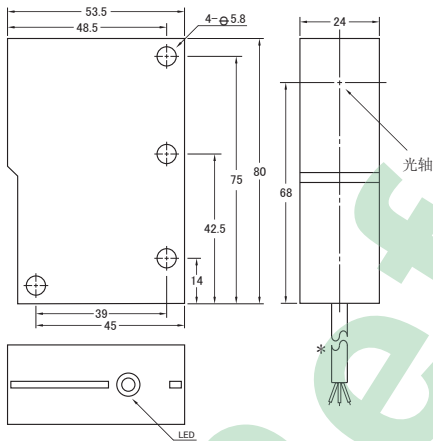
图191 HDT500-24K-□ HDM80-24K-□ HDR200-24K-□
